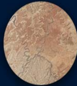
Lithosphere
